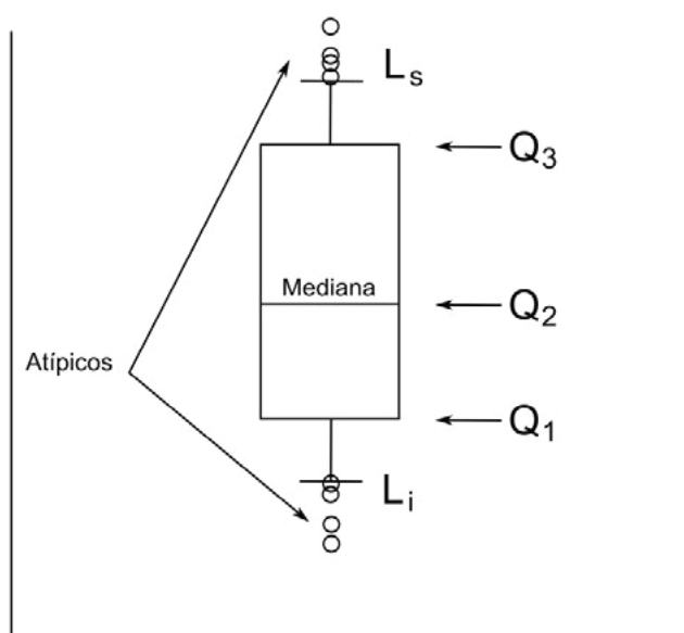
Figura 6 – Box plot
