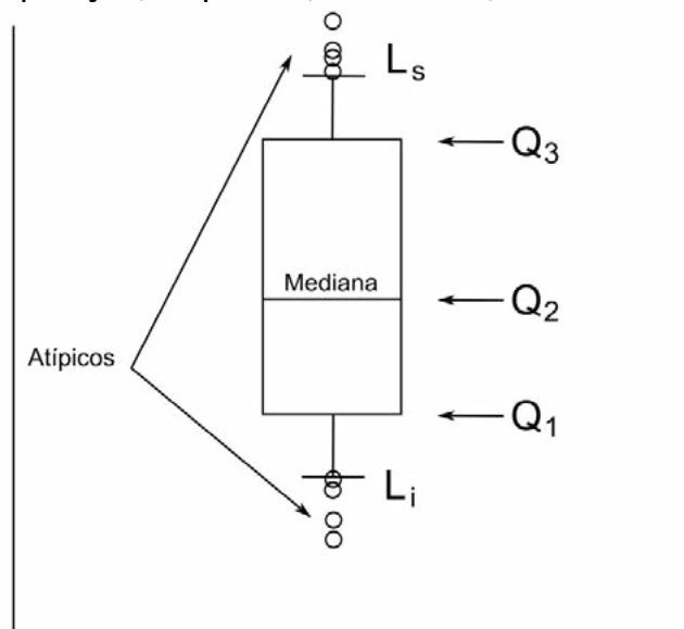
Figura 6 – Box plot
